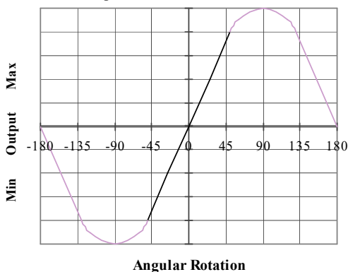
Output Characteristic - Standard
